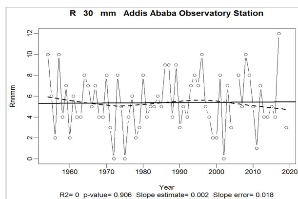
Figure 12: Heavy precipitation days for Addis Ababa observatory station (precipitation > 30 mm)
