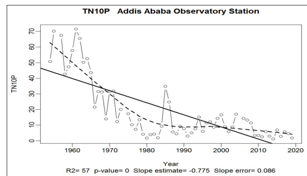
Figure 18: Days with T_{\min} < 10^{\text{th}} percentile of daily minimum temperature (cold nights)-Addis Ababa observatory station
