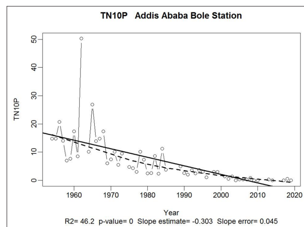
Figure 17: Days with T_{\min} < 10^{\text{th}} percentile of daily minimum temperature (cold nights)-Addis Ababa Bole
