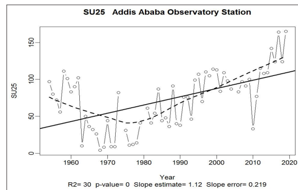
Figure 16: Frequency of days when Tmax > 25°C for Addis Ababa observatory station
