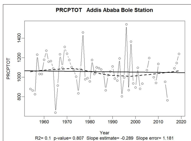
Figure 3: Addis Ababa Bole Station's yearly total precipitation in rainy days (rain greater than 1 mm).
