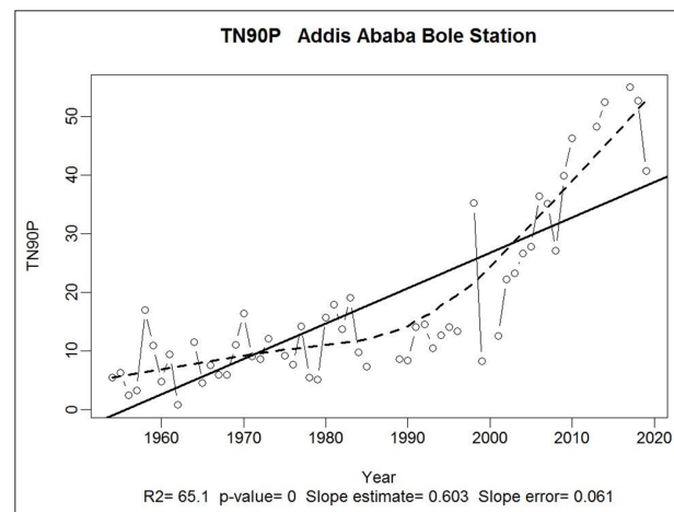
Figure 23: Days with T_{\min} > 90^{\text{th}} percentile of daily temperature (warm nights)-Addis Ababa-Bole station
