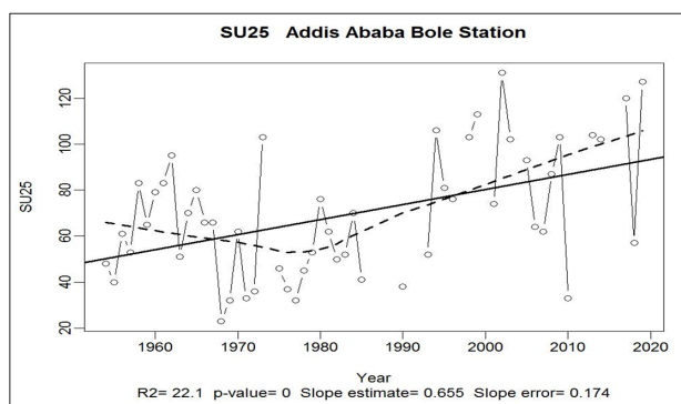
Figure 15: Frequency of days when Tmax > 25°C for Addis Ababa Bole station
