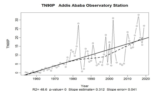
Figure 24: Days with T_{\min} > 90^{\text{th}} percentile of daily temperature (warm nights)-Addis Ababa-observatory station
