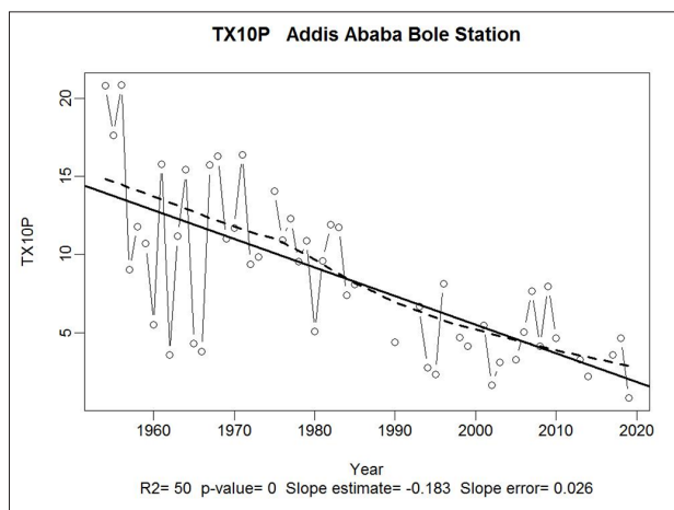
Figure 19: Days with T_{\max} < 10^{\text{th}} percentile of daily maximum temperature (cold day)-Addis Ababa bole station
