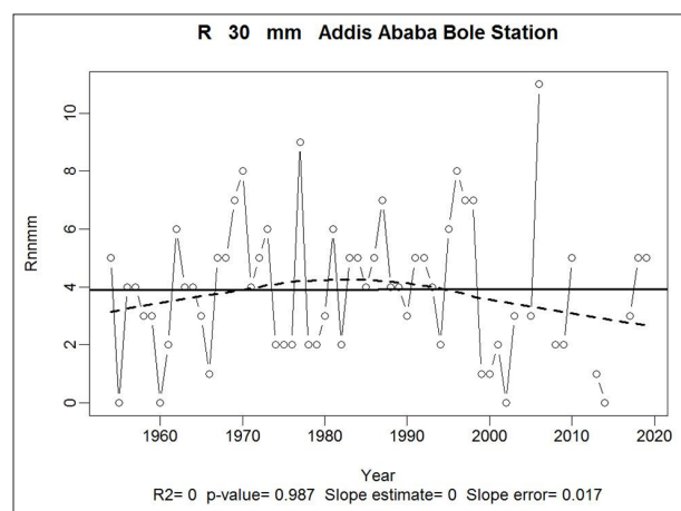
Figure 11: Heavy precipitation days for Addis Ababa Bole station (precipitation > 30 mm)
