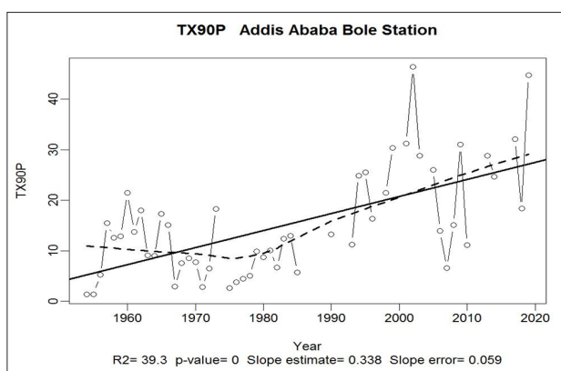
Figure 21: Days with T_{\max} > 90^{\text{th}} percentile of daily maximum temperature (warm daytimes)-Addis Ababa Bole station.
