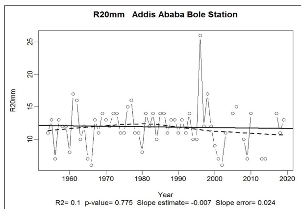
Figure 9: Heavy precipitation days for Addis Ababa Bole station (precipitation > 20 mm)
