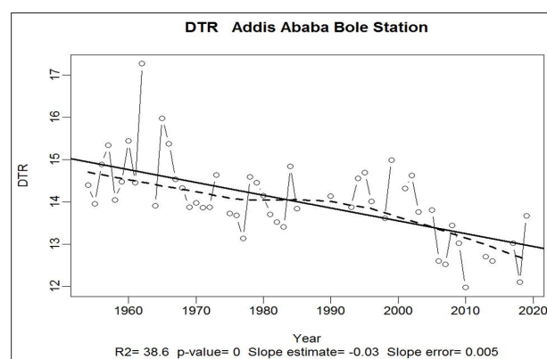
Figure 27: Mean of diurnal temperature range (°C)-Addis Ababa Bole station
