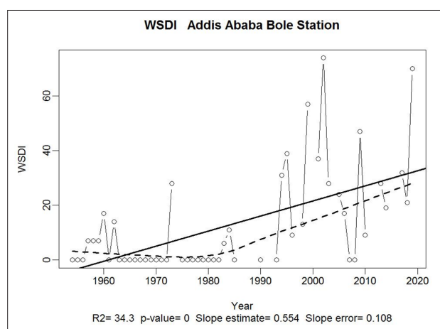
Figure 25: Warm spell duration (days)-Addis Ababa Bole station
