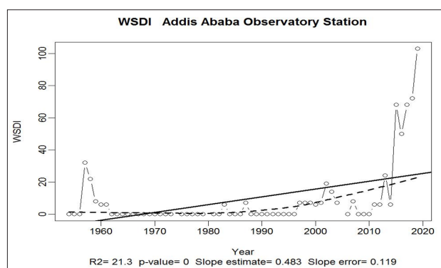
Figure 26: Warm spell duration (days)-Addis Ababa observatory station
