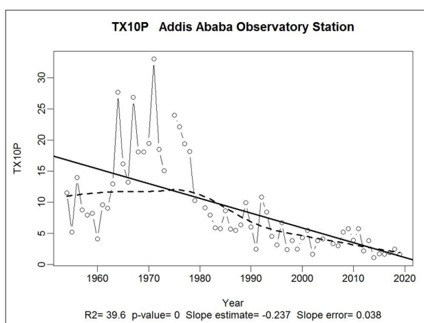
Figure 20: Days with T_{\max} < 10^{\text{th}} percentile of daily maximum temperature (cold day)-Addis Ababa observatory station
