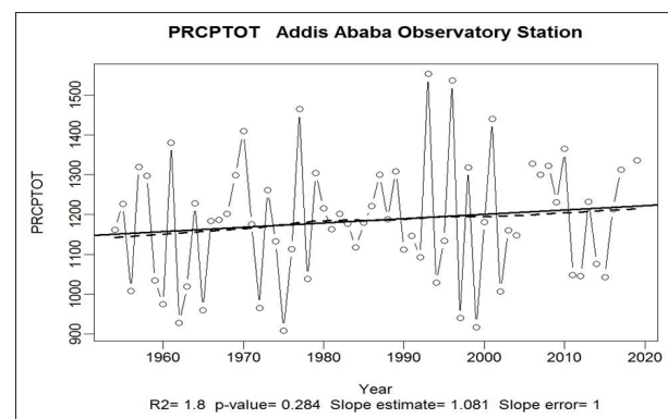
Figure 4: Annual total precipitation for Addis Ababa Observatory on wet days (rain greater than 1 mm)
