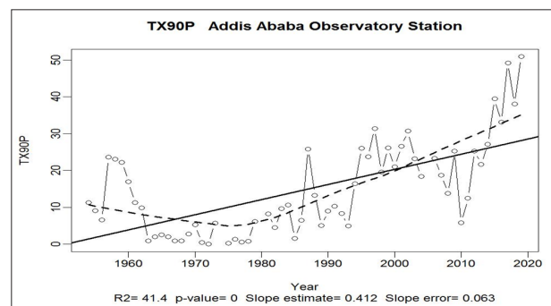
Figure 22: Days with T_{\max} > 90^{\text{th}} percentile of daily maximum temperature (warm day-times)-Addis Ababa observatory station
