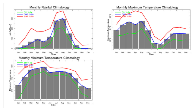
Figure 2: shows the climatology of Addis Ababa's monthly rainfall, maximum temperature, and lowest temperature
