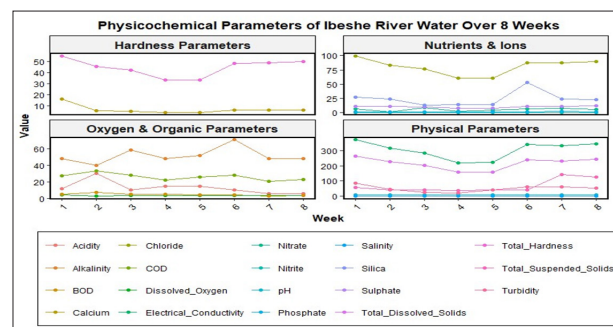
Figure 3: Temporal variation in physicochemical parameters of Ibeshe River water over an 8-week sampling period. Panels show (A) physical parameters (pH, electrical conductivity, TSS, TDS, turbidity, salinity), (B) oxygen and organic parameters (DO, BOD, COD, acidity, alkalinity), (C) nutrients and ions (chloride, nitrate, nitrite, sulphate, phosphate, silica), and (D) hardness parameters (total hardness, calcium). Note the distinct y-axis scales reflecting different measurement units and concentration ranges
