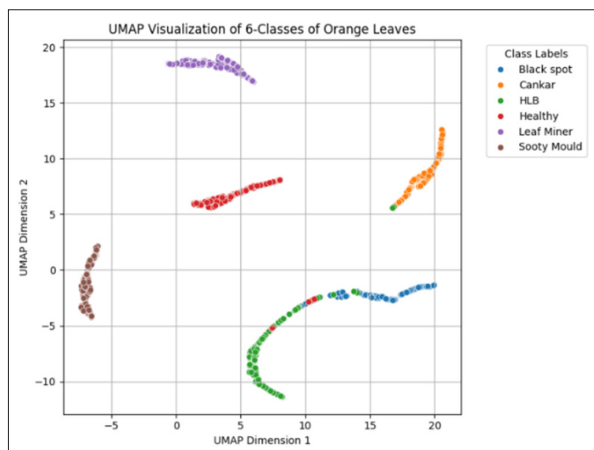
Figure 10: UMAP of MobileNetV2
