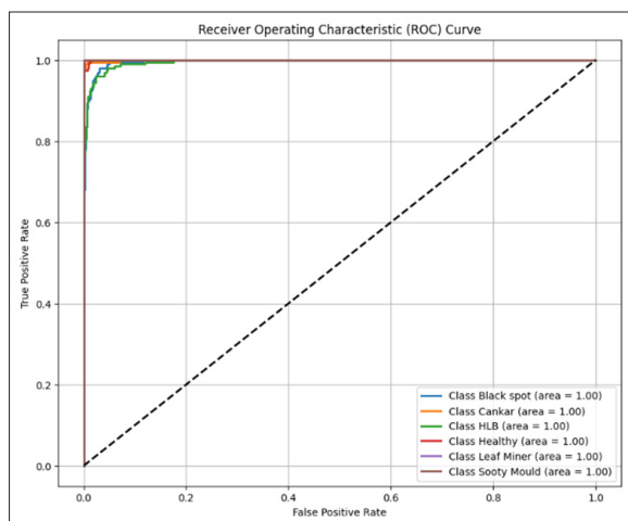
Figure 6: ROC curve of MobileNetV2
