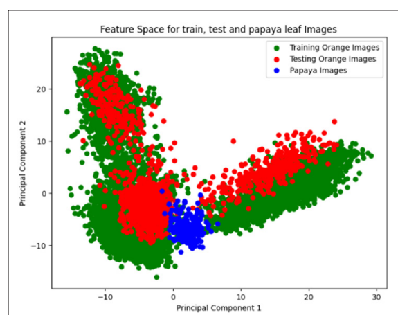
Figure 3: Feature Space with Train, Test and Additional Image
