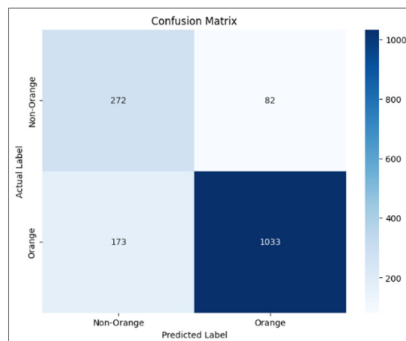
Figure 2: Confusion Matrix of One-Class SVM
