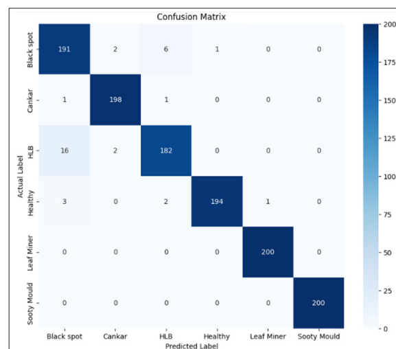
Figure 7: Confusion Matrix of MobileNetV2
