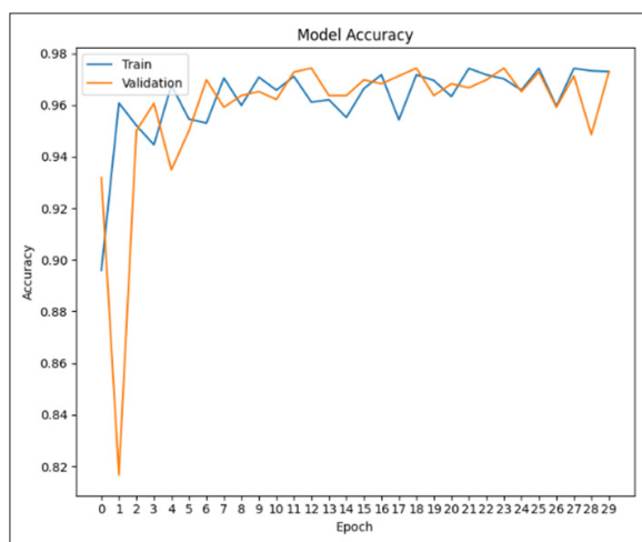
Figure 4: Accuracy graph of Inceptionv3
