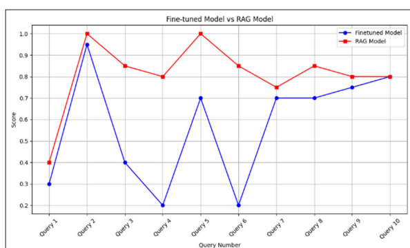
Figure 11: Chatbot Evaluation Line Graph
