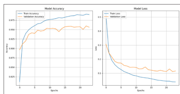
Figure 9: Accuracy and Loss plots of MobileNetV2
