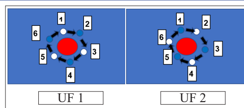
Figure 2: "G-D's Physics" Alternative Explanation for "Curved Space-Time"!
