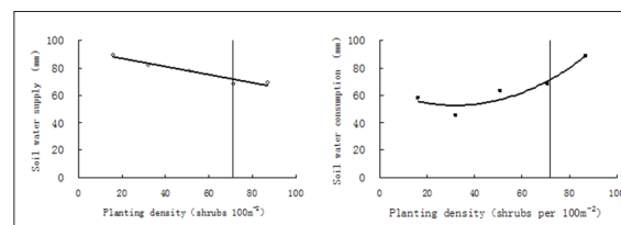
Figure 4: The changes of soil water supply and soil water consumption with planting density and SWVCC in the key period of plant water relation regulation of Caragana shrubland of the semiarid loess hilly region, China. a, The change in soil water supply with planting density and SWVCC; b, The change in Soil water consumption with planting density and SWVCC.
