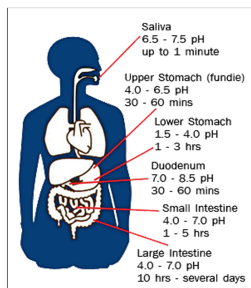
Figure 1: GI PH variation
